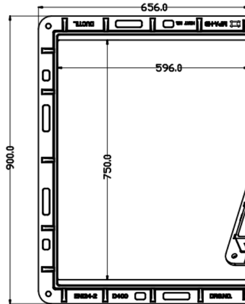
FRAME PART
