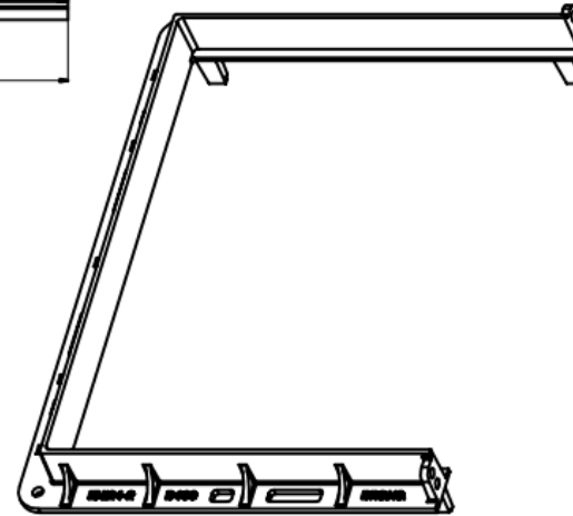
FRAME PART
